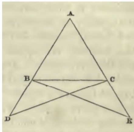
FIRST FORMULA. The sums of equals are equal.
